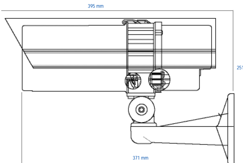
Housing and bracket assembly dimension (mm)
